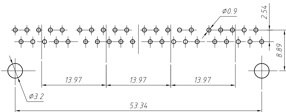
PCB Layout
